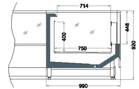
PLATIN DW 2060 / HC Length mm | 1948
